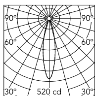
Luminous flux luminaire 121 lm
