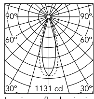
Luminous flux luminaire 409 lm
