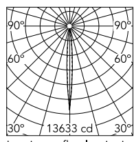
Luminous flux luminaire 535 lm
