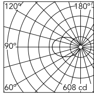
Luminous flux luminaire 580 lm
