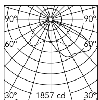
Luminous flux luminaire 3173 lm
