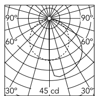
Luminous flux luminaire 74 lm
