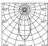
Luminous flux luminaire 1610lm
