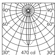
Luminous flux luminaire 110 lm
