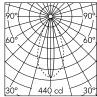
Luminous flux luminaire 103 lm
