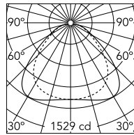
Luminous flux luminaire 4441 lm (EXTREME CUT OFF)
