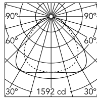
Luminous flux luminaire 4622 lm (EXTREME CUT OFF)
